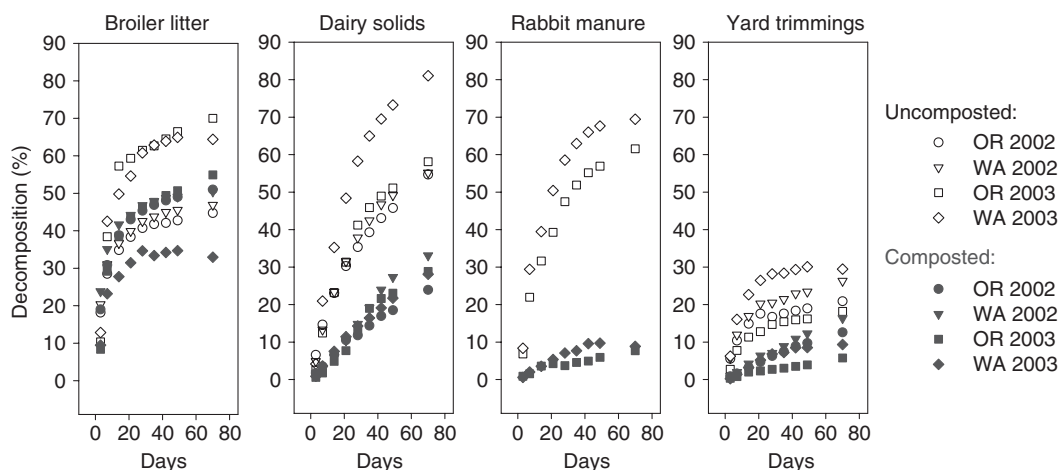
Fig. 1. Cumulative decomposition in the laboratory at 22°C for organic amendments incubated in soils from Washington (WA) and Oregon (OR) field sites in 2002 and 2003. Open symbols represent uncomposted organic amendments, whereas filled symbols represent amendments that were “composted.” Fitted regression equations for cumulative decomposition of each amendment are shown in Table 3.
