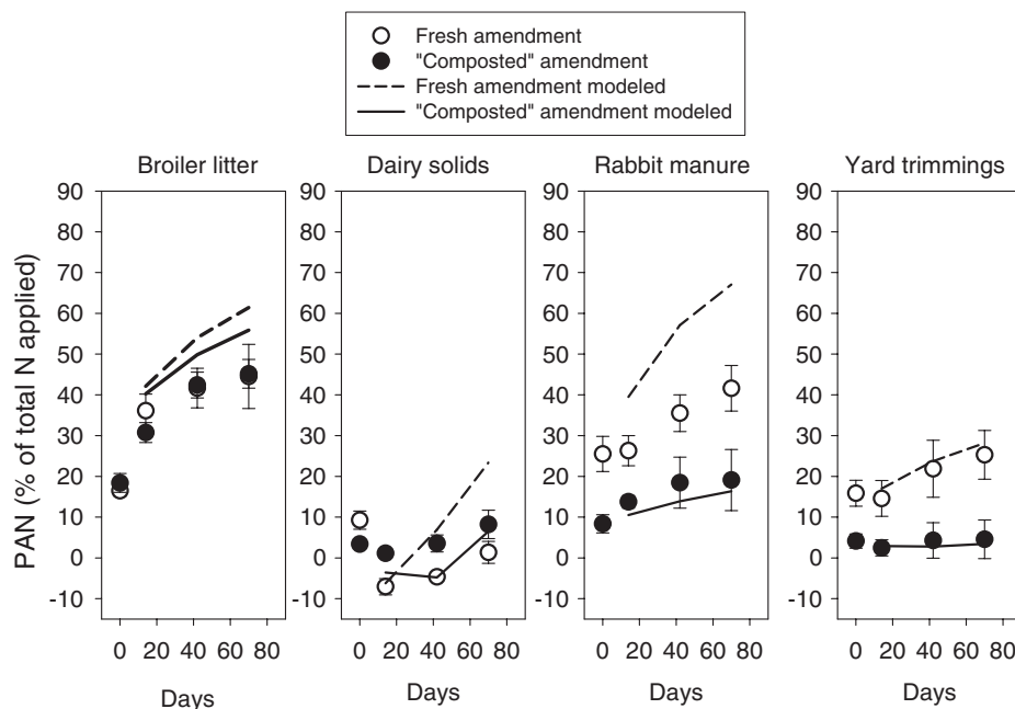
Fig. 4. Observed and modeled PAN for laboratory incubations of amendments included in the fresh vs. “composted” product comparison. Data points represent averages across soils and years ( n = 2 for rabbit manure; n = 4 for others). Error bar is standard error of the mean computed across soils and years. Point estimates of PAN were estimated by the DECOMPOSITION model for 14, 42, and 70 d of incubation at 22°C.
