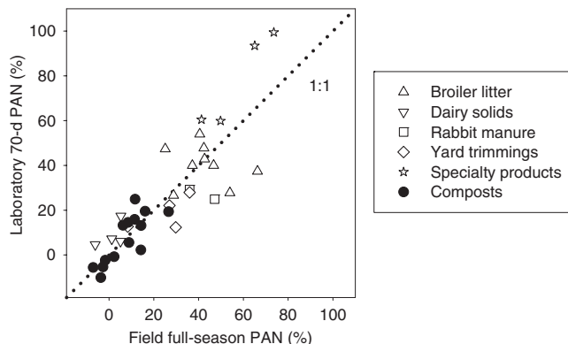
Fig. 2. Plant-available nitrogen (PAN) observed for the full season in the field vs. PAN observed at 70 d in laboratory incubations at 22°C.
