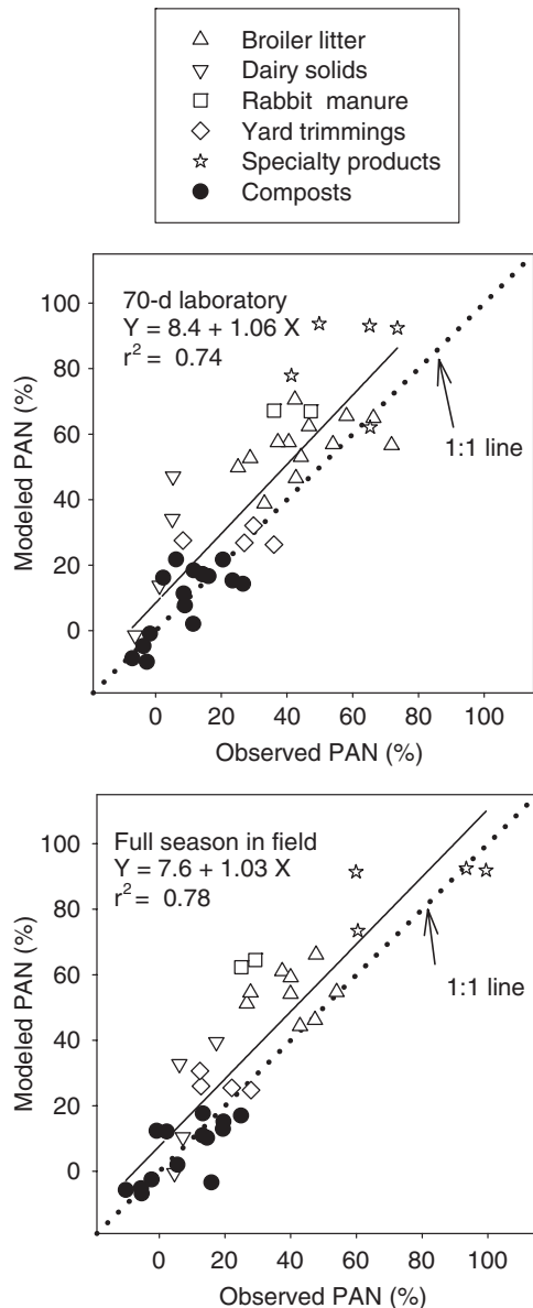
Fig. 5. Observed and modeled PAN for laboratory incubation at 22°C and for full-season field trials. Dotted line is 1:1 line.
