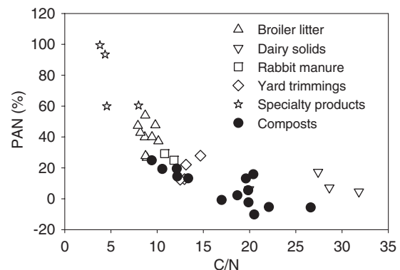
Fig. 3. Relationship between full-season PAN in field trials and organic amendment C/N.
